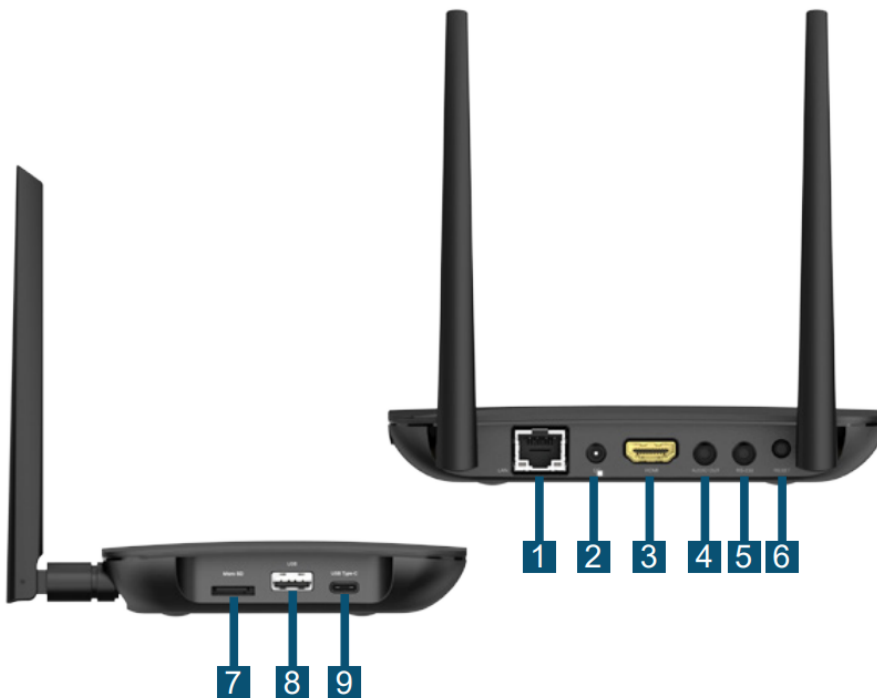
Hardware Ports
