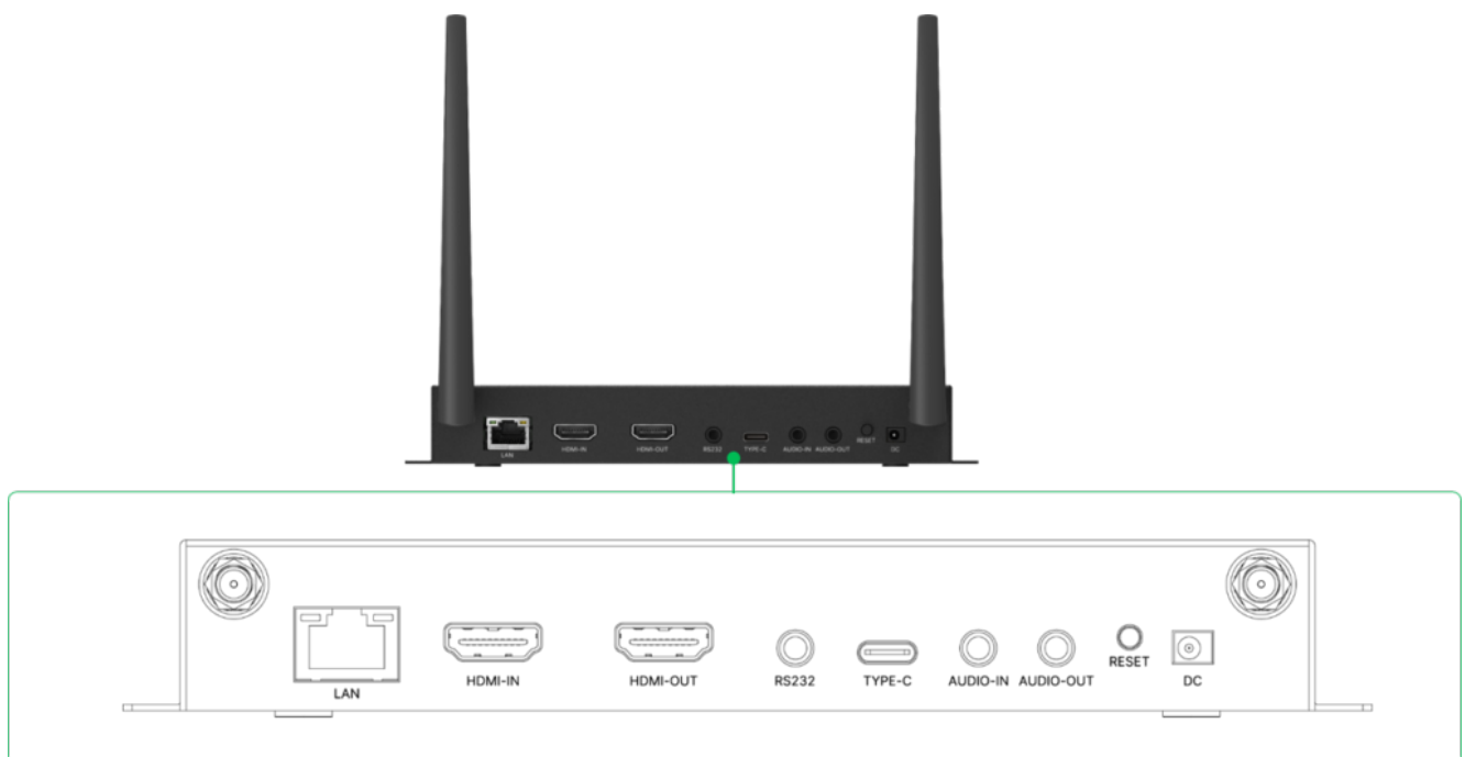
NC-X710 & NC-X910 back I/O ports in back side
